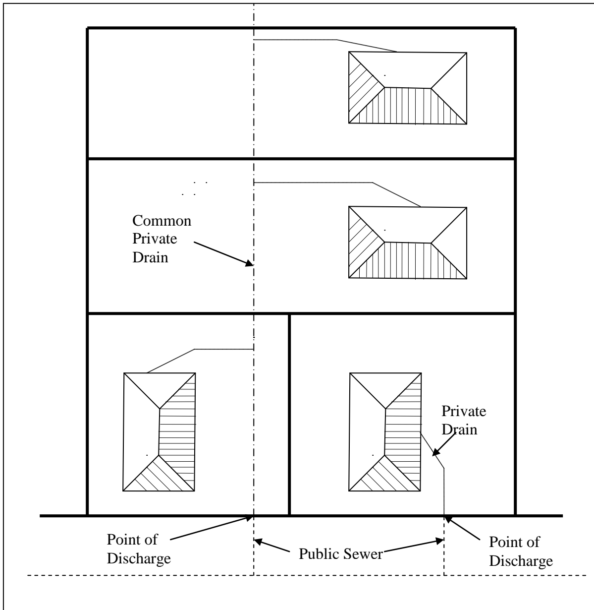
Figure 4 - Point of Discharge Location - Common Private Drain
