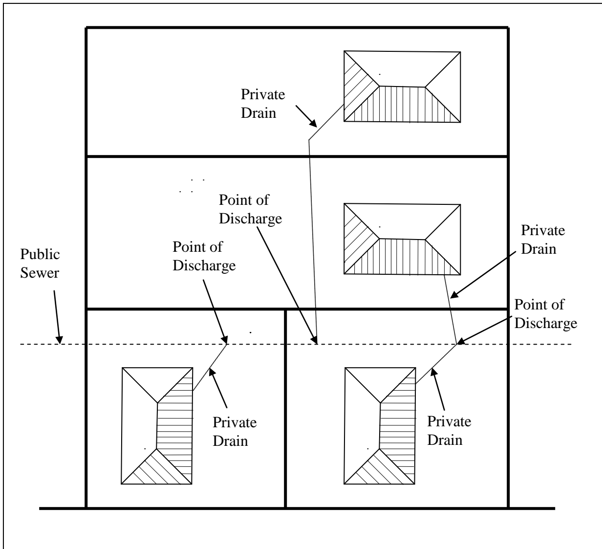
Figure 5 - Point of Discharge Location - Private Drain through Neighbouring Properties
