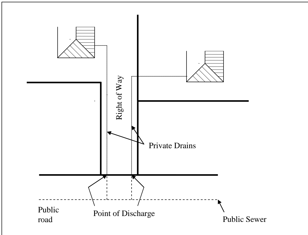
FIGURE 1 - POINT OF DISCHARGE LOCATION - WITH STREET FRONTAGE
